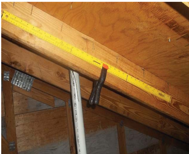
Roof decking method of attachment
