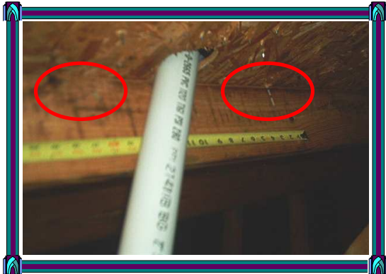
The following three pages of pictures show the numerous missed studs in the attic.
